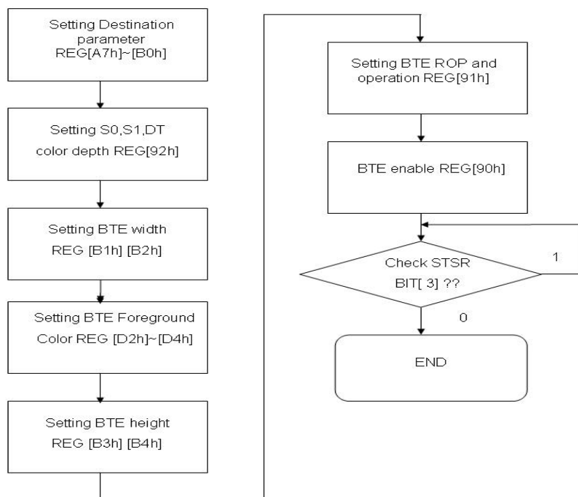
Figure 4-3 : Flow Chart
