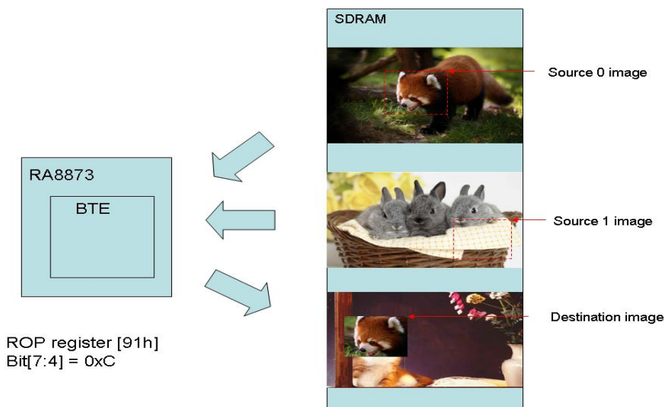
Figure 4-27 : Hardware Data Flow
