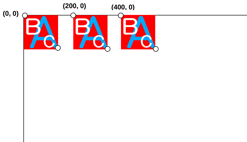
Figure 1.6 : 16 bits MCU and 24bpp color depth mode2 MCU Write data to SDRAM(Layer1)
