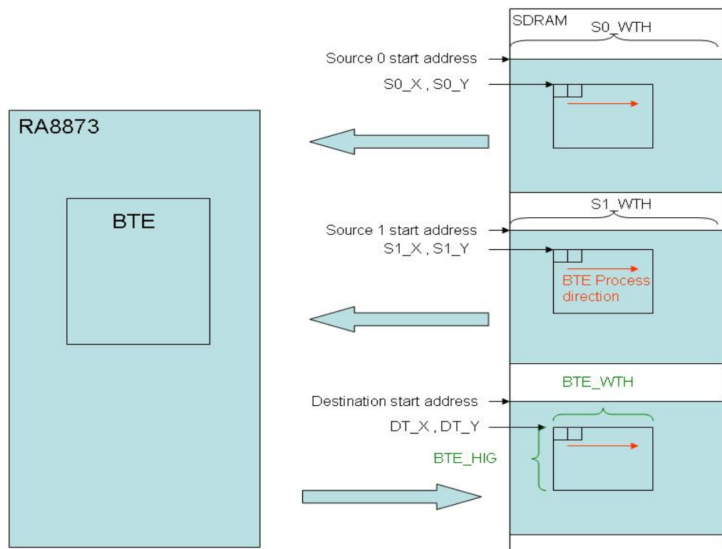
Figure 4-1 : Memory Access of BTE Function
