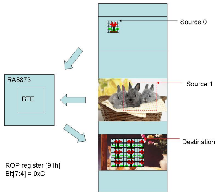
Figure 4-72 : Hardware Data Flow
