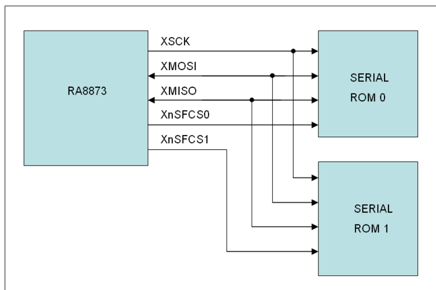
Figure 3.3: RA8873 Serial Flash/ROM System
